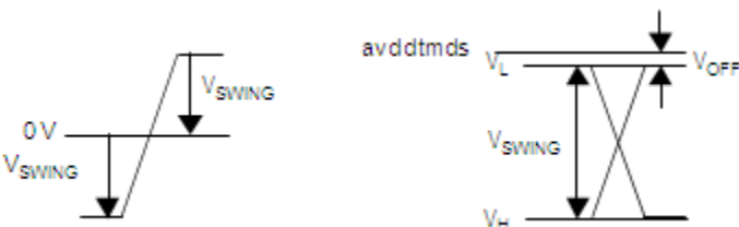
Figure 52. Driver Definitions
