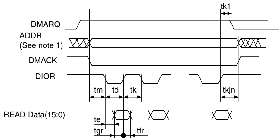
Figure 13. MDMA Read Mode Timing
