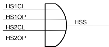
Figure 46. High-side status
