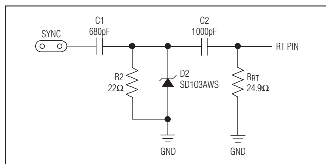
Figure 1. SYNC Circuit
