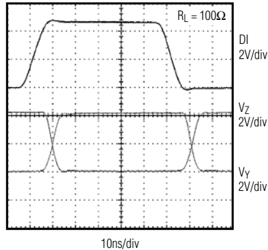
DRIVER PROPAGATION DELAY (16Mbps)
