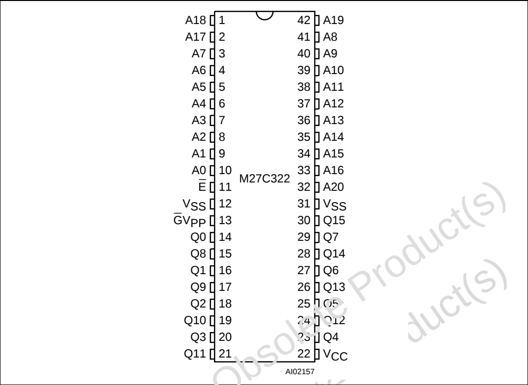
Figure 2. DIP Connections
