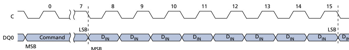
Figure 14: WRITE STATUS REGISTER Command Sequence
