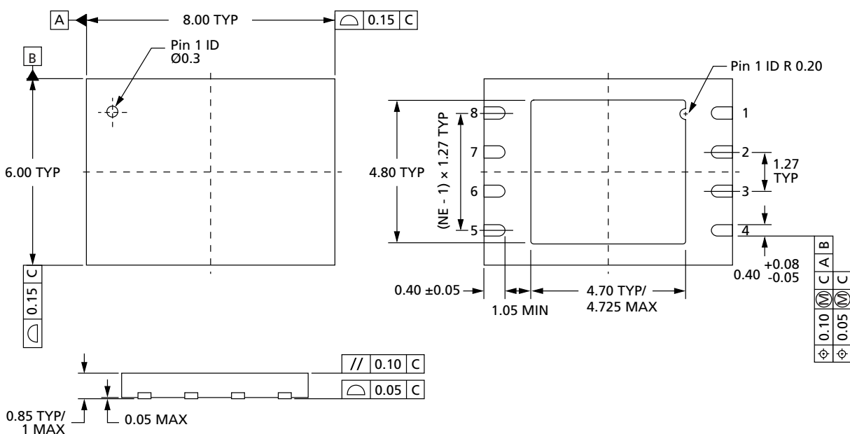
Figure 38: VDFPN8 (MLP8, MD) 6mm x 8mm with Reduced D2 Dimension
