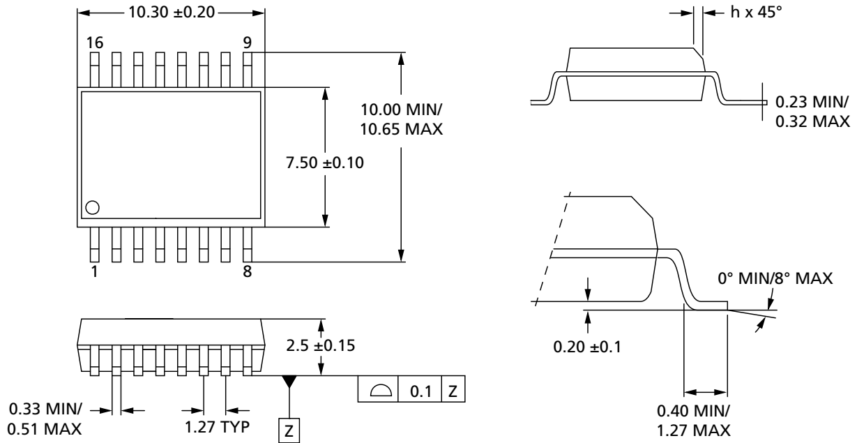
Figure 31: SO16W 300 mils Body Width
