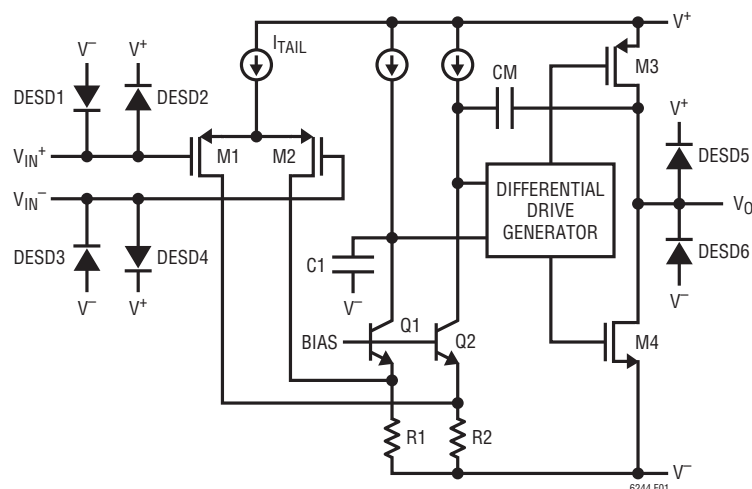
Figure 1. Simplified Schematic
