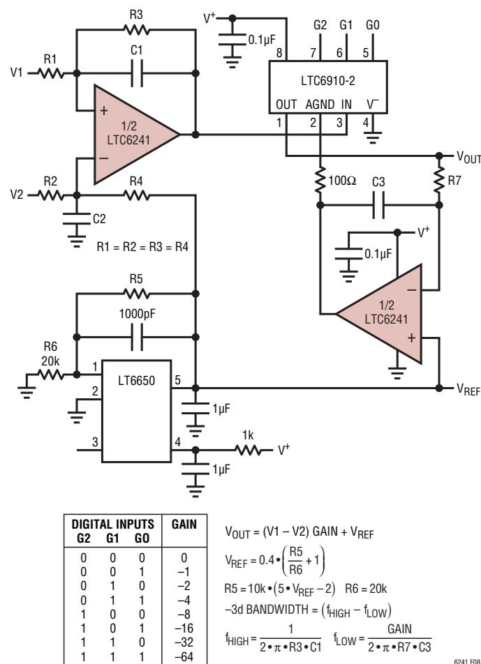
Figure 8. Wideband Difference Amplifier with High Input Impedance and Digitally Programmable Gain
