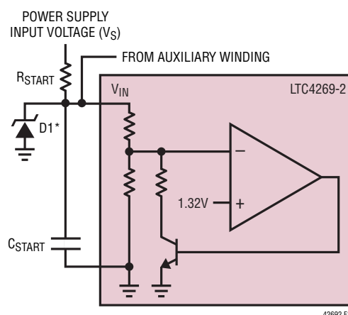
Figure 9. Programming Power Supply Undervoltage Lockout (UVLO)
