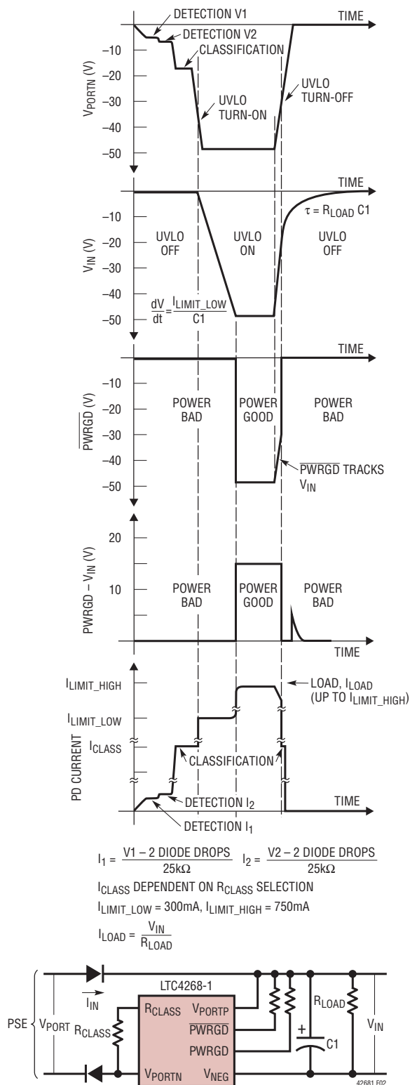
Figure 2. V_{IN} Voltage, \overline{\text{PWRGD}} , \overline{\text{PWRGD}} and PD Current as a Function of Port Voltage
