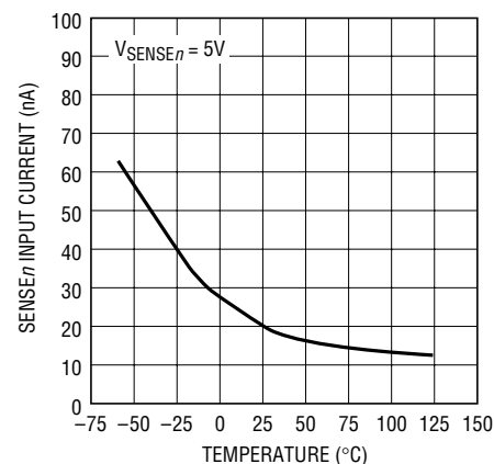
SENSE_n Input Current vs Temperature
