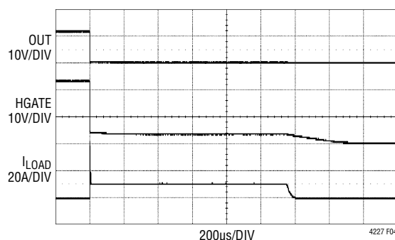
Figure 4. Overcurrent Fault on 12V Output
