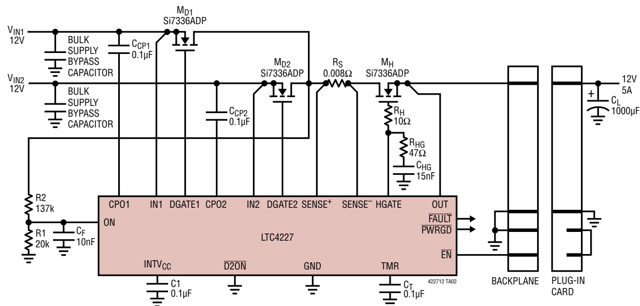
Backplane Resident Diode-OR Application with Inrush Current Limiting at 12V Supply Inputs
