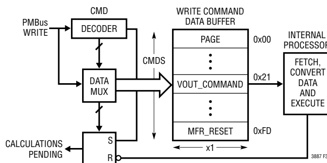
Figure 37. Write Command Data Processing
