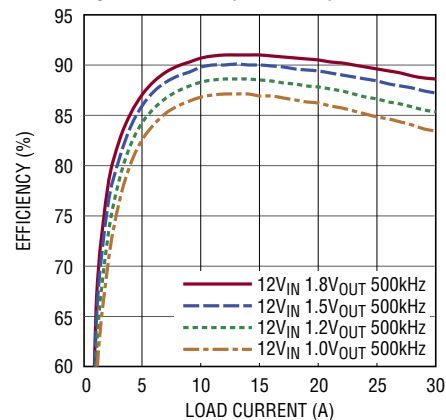
Efficiency vs Load Current F SW = 500kHz (LTC3887)
