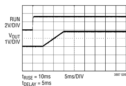
Soft-Start Ramp
