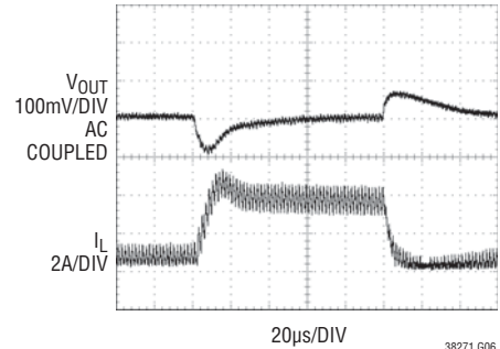
FIGURE 13 CIRCUIT V_{OUT} = 3.3V
