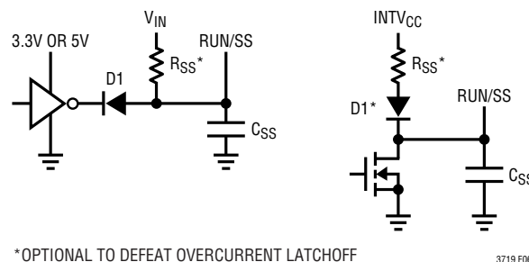
Figure 5. RUN/SS Pin Interfacing
