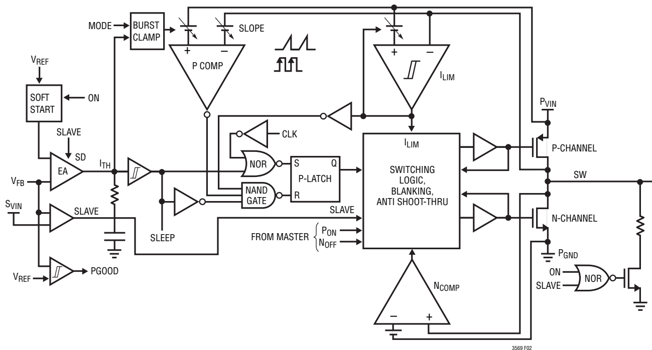
Figure 2. Buck Block Diagram
