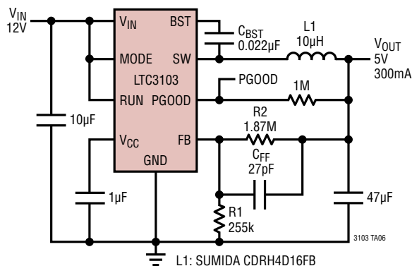
12V to 5V/300mA Regulator with High Efficiency, Ultralow I Q (1.8μA with V OUT in Regulation, No Load)
