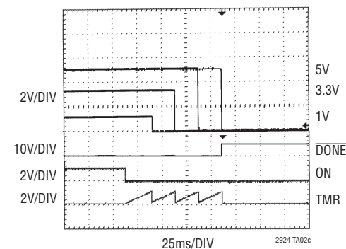
Power-Down Sequence
