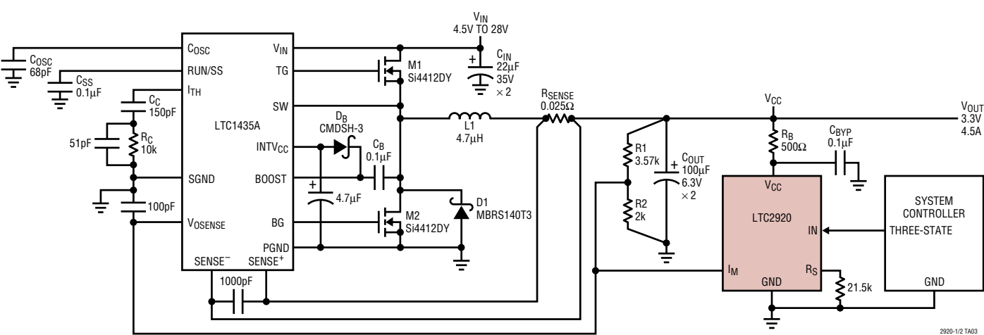
3.3V Supply with ±0.165V (5%) Voltage Margining
