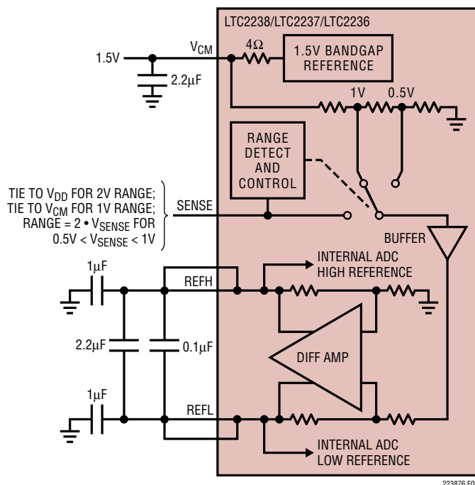
Figure 9. Equivalent Reference Circuit
