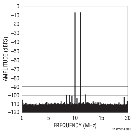
LTC2141-14: 64k Point 2-Tone FFT, f_{IN} = 69\text{MHz} , 70\text{MHz} , -7\text{dBFS} , 40Msps
