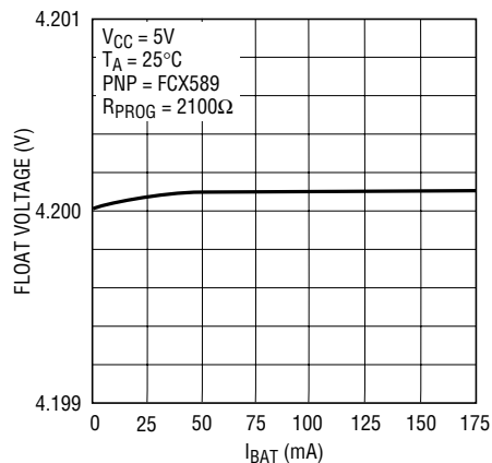
Float Voltage vs I_{BAT}
