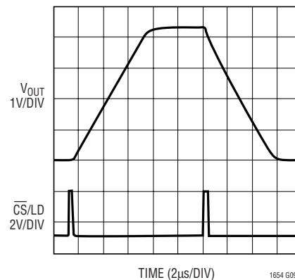
Large-Signal Settling—Slow Mode
