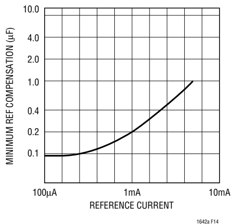
Figure 14. Minimum REF Compensation vs REF Current
