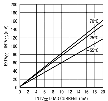
EXTVC CC Switch Drop vs INTV CC Load Current
