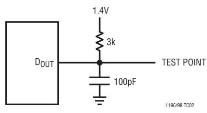
Load Circuit for t dD0 , t r and t f
