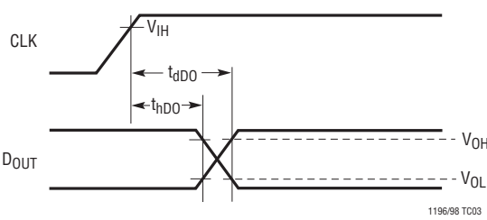
Voltage Waveform for D OUT Delay Time, t dD0 , t hD0
