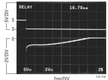
Negative Overload Recovery
