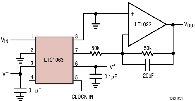
Figure 3. Test Circuit for THD
