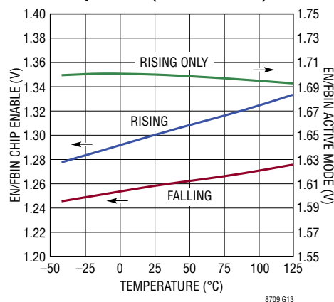
EN/FBIN Thresholds vs Temperature (1.7V and 1.3V)
