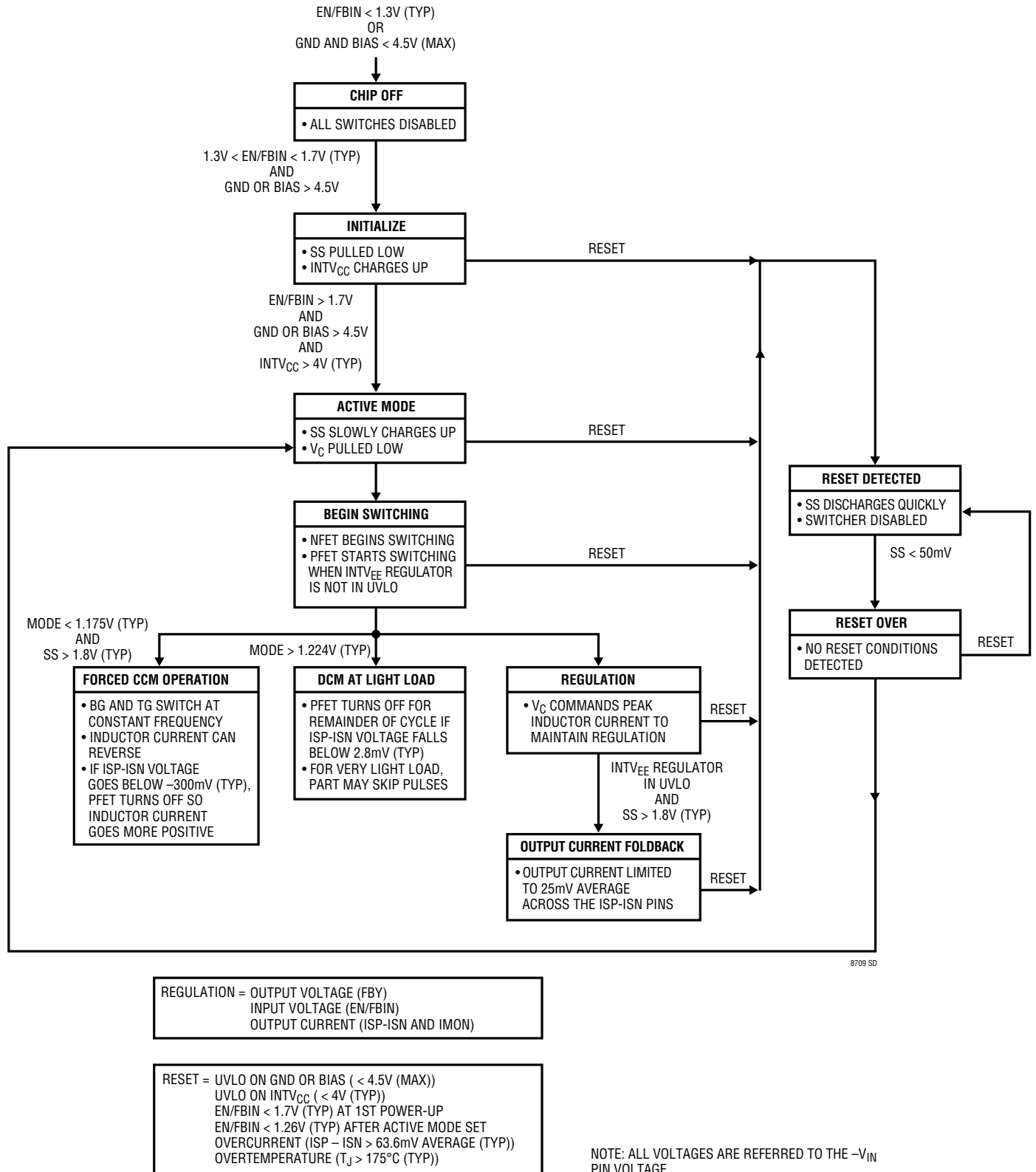
Figure 2. State Diagram
