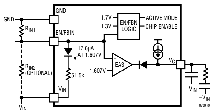
Figure 9. Configurable UVLO
