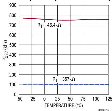
Oscillator Frequency vs Temperature (100kHz and 750kHz)
