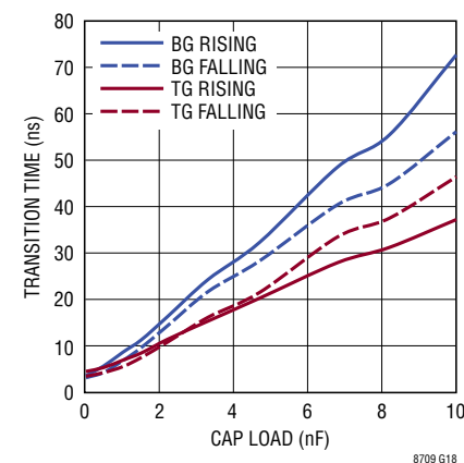
BG and TG Transition Time vs Cap Load
