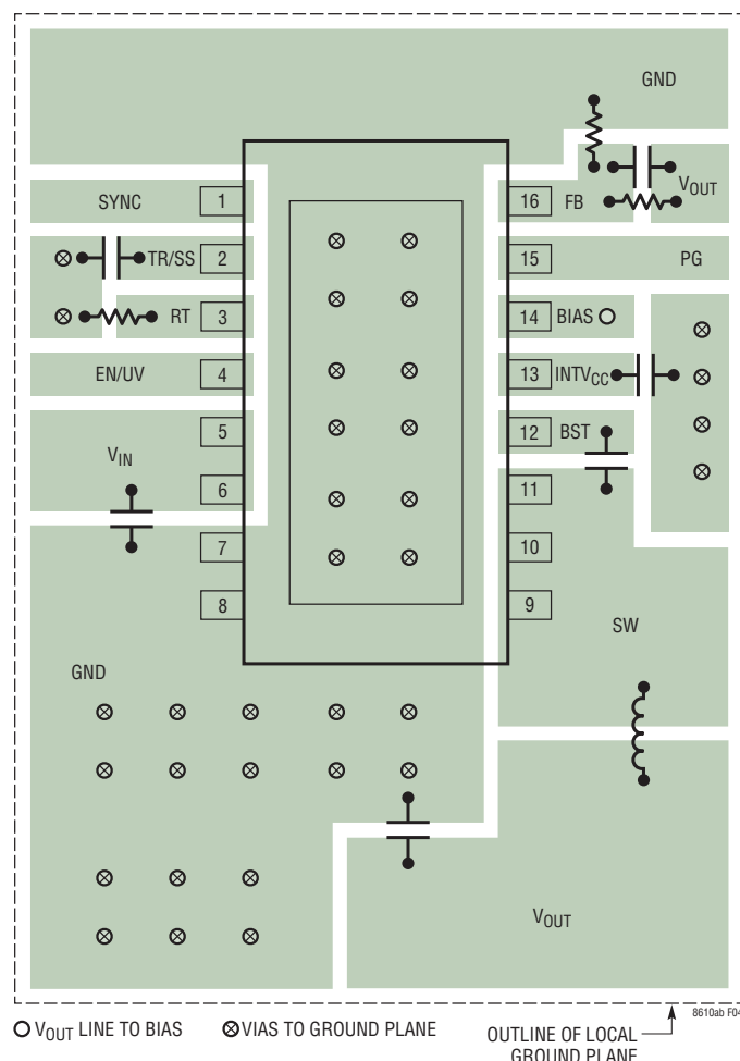
Figure 4. Recommended PCB Layout for the LT8610A/LT8610AB
