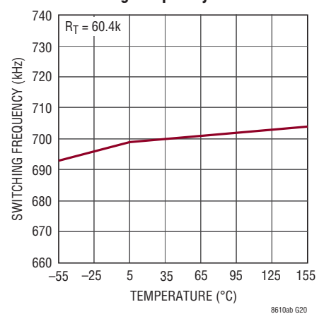
Switching Frequency
