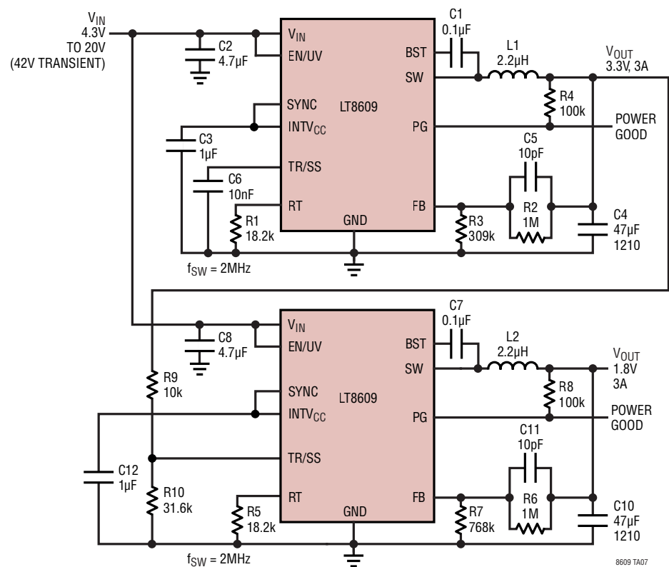
Tracking 3.3V and 1.8V 2MHz Converters
