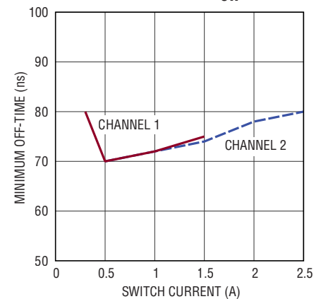
Minimum Off-Time vs I_{SW}
