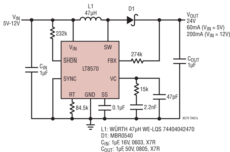
1MHz Boost Converter Generates 24V from 5V-12V Input
