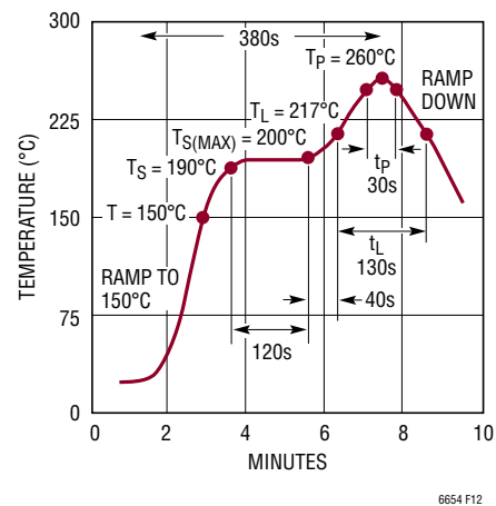
Figure 12. Lead Free Reflow Profile
