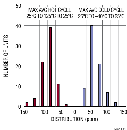
(a) LT6654 S6 Thermal Hysteresis -40^{\circ}\text{C} to 125^{\circ}\text{C}
