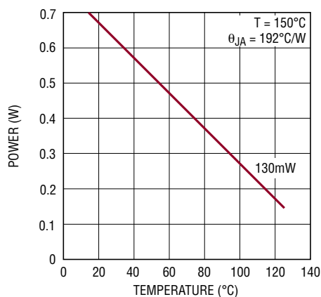
Figure 9. Maximum Allowed Power Dissipation of the LT6654
