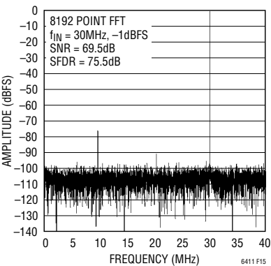
Figure 15. SNR and SFDR of the LT6411 and Filter Driving the LTC2249
