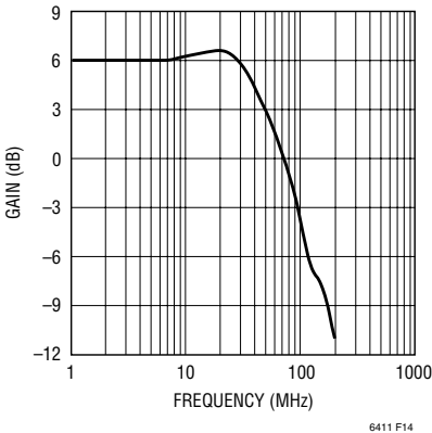
Figure 14. Frequency Response of the LT6411 and Filter
