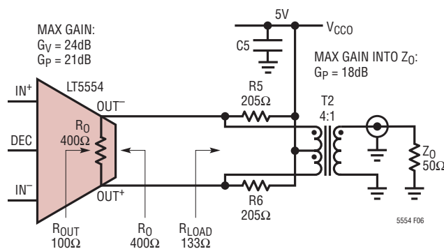
Figure 6. Single-Ended Matched Output Interface
