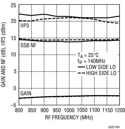
Figure 4. Typical Gain, IIP3 and NF with Series 3.9pF Matching Capacitor
