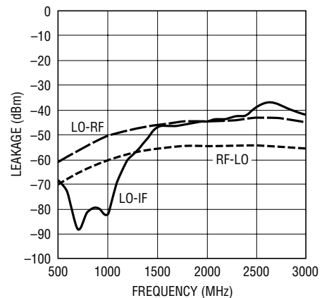
LO-IF, LO-RF and RF-LO Leakage vs Frequency
