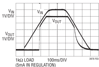
Figure 3. V_{IN} to V_{OUT} Performance
