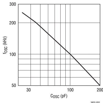
Figure 2. f_{\text{OSC}} vs OSC Capacitor Values
