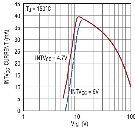
INTV CC Minimum Output Current vs V_{IN}
