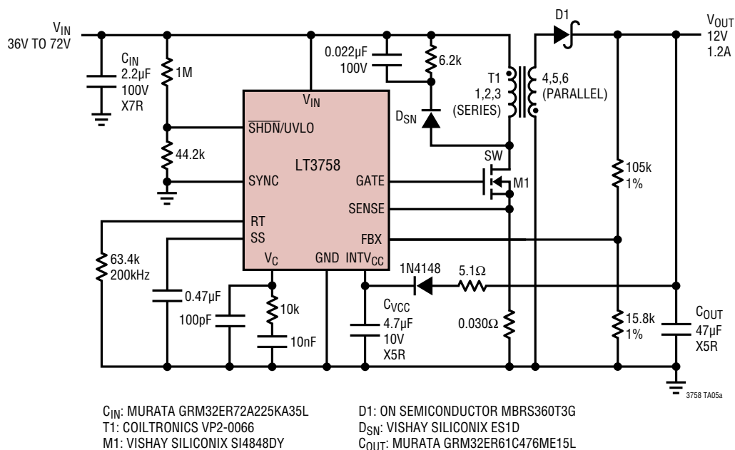
12V Output Nonisolated Flyback Power Supply
