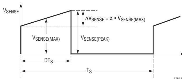
Figure 2. The Sense Voltage During a Switching Cycle
