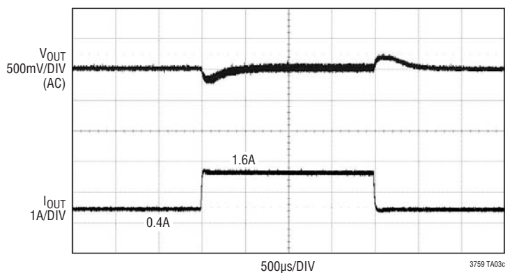
Load Step Response at V_{IN} = 12V
