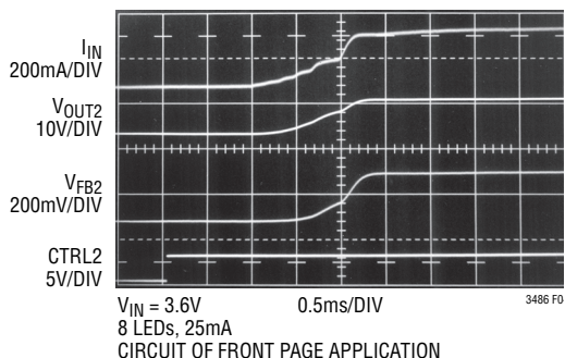
Figure 4. Start-Up Waveforms
