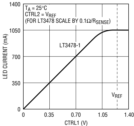
LED Current vs CTRL1
