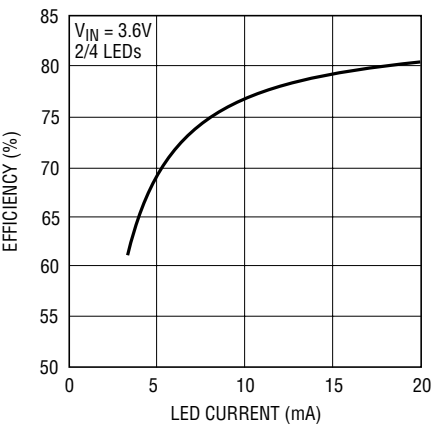
Conversion Efficiency
