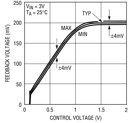
Distribution of V_{FB} vs V_{CTRL}
