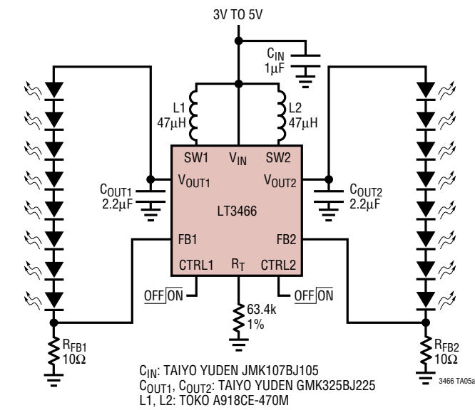
Li-Ion to 8/8 White LEDs
