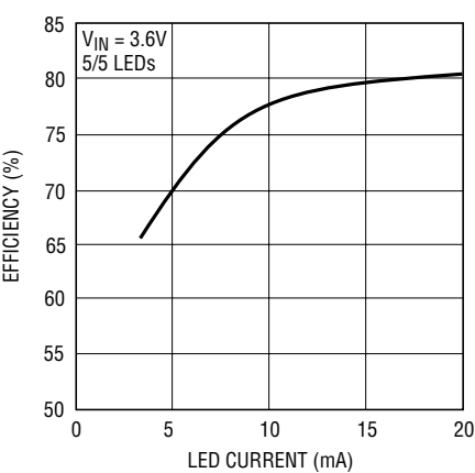
Conversion Efficiency
