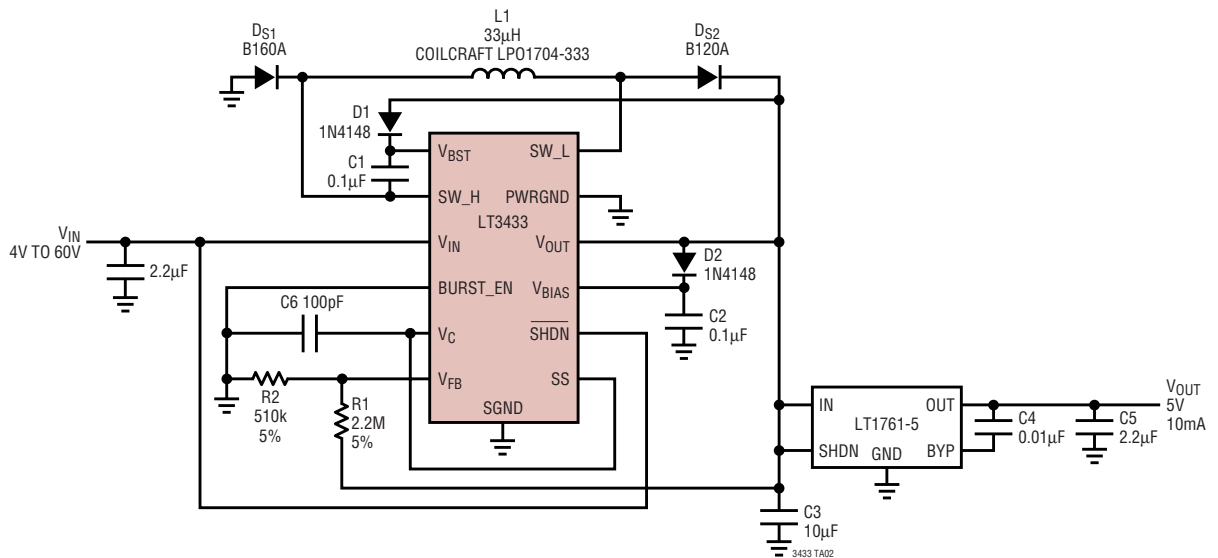
Burst Only Low Noise 5V Maintenance Supply
