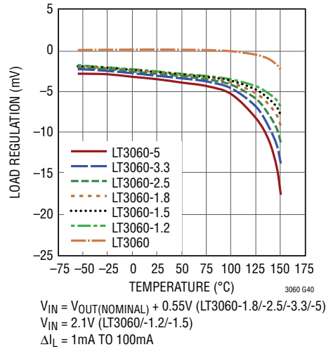
Load Regulation
