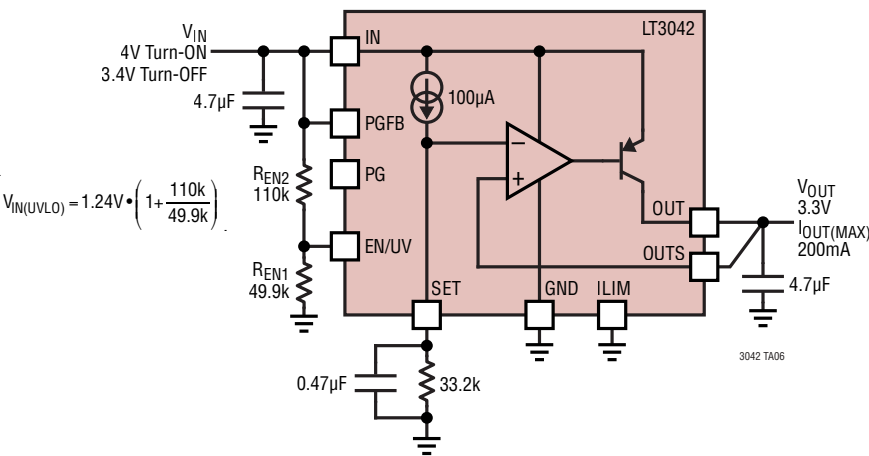
Programming Undervoltage Lockout
