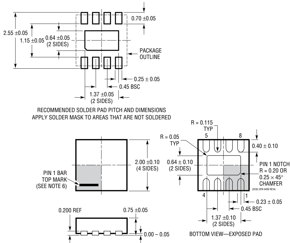
DC Package 8-Lead Plastic DFN (2mm × 2mm) (Reference LTC DWG # 05-08-1719 Rev A)
